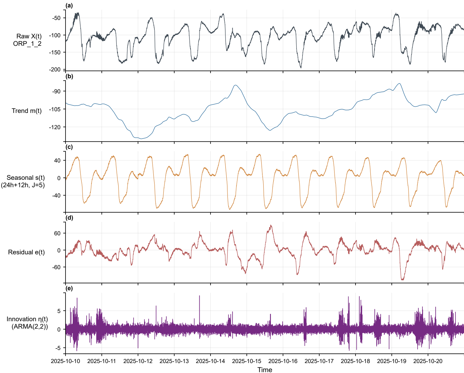
Multi-scale decomposition — ORP_1_2 (pre_anoxic_front, min) [2025-10-10~2025-10-20]
